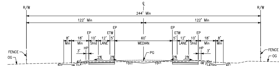
TYPICAL SECTION INTERIM
