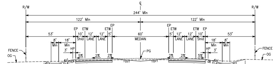
TYPICAL SECTION ULTIMATE
